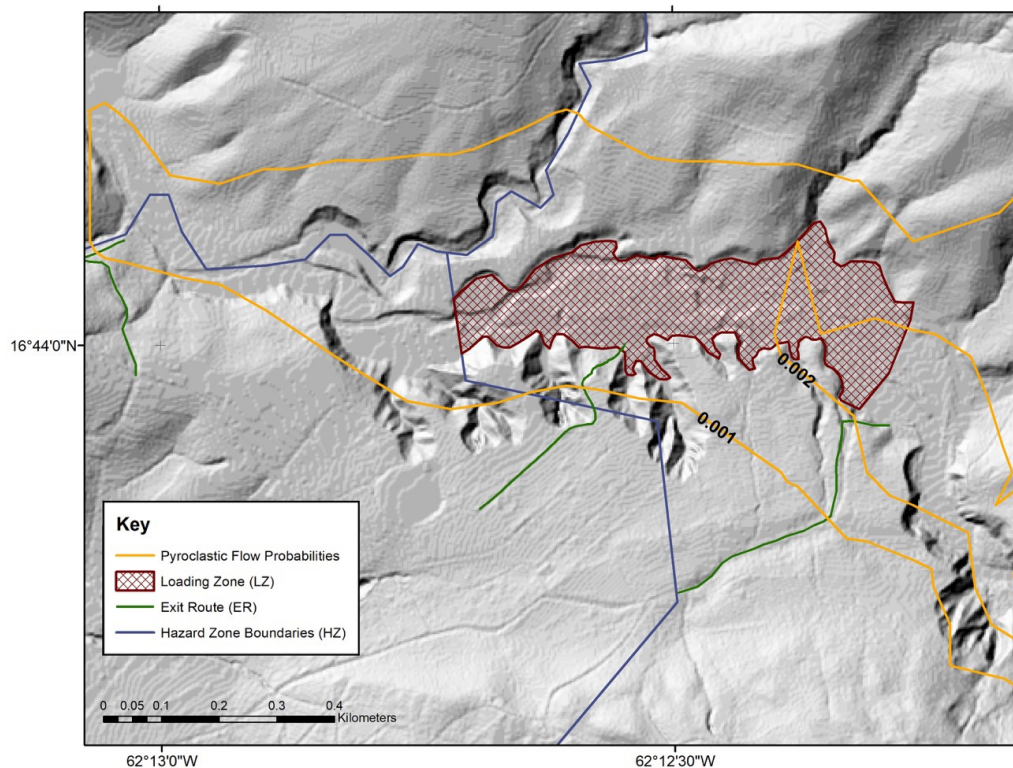
Figure 3: Probabilities of pyroclastic flow impact areas in the Upper Belham Valley for a five-year timeframe. The spatial distributions are modelled by combining flow simulations undertaken in TITAN2D (Patra et al., 2005) with the statistical analysis of historical events.
