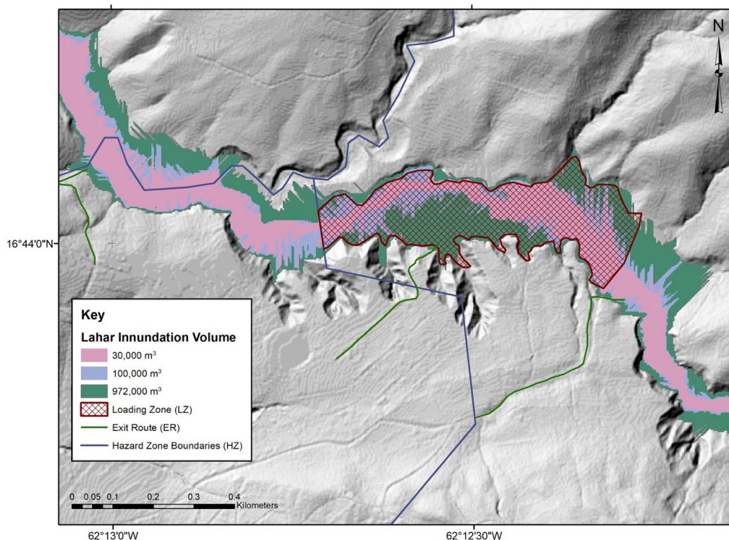
Figure 2: Potential lahar inundation areas in the Upper Belham Valley. The lahar hazard footprints are calculated using the computational modelling tool LAHARZ (Schilling, 1998) using the upper limit volumes from each category of lahar. Loading Zone (LZ) coordinates, and Exit Route (ER) locations were provided by the Physical Planning Unit (PPU) of Government of Montserrat.
